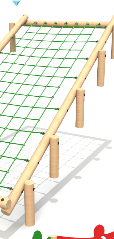
Large Embankment Net L 5050 W 2800 H 825mm FFH 825mm
